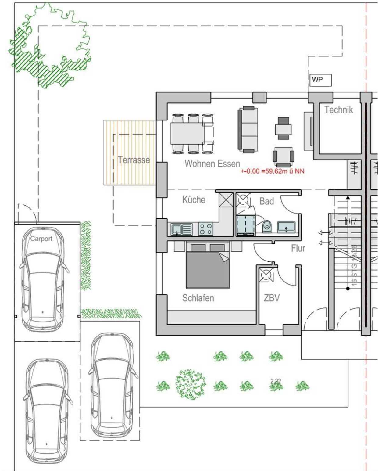
Erdgeschoss links
