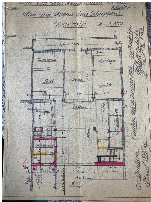
Scheune Grundriß
