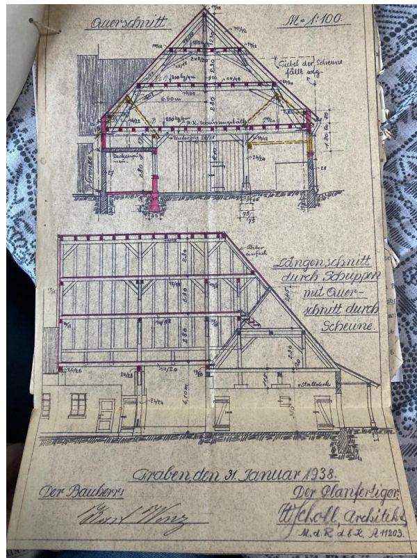
Scheune Plan
