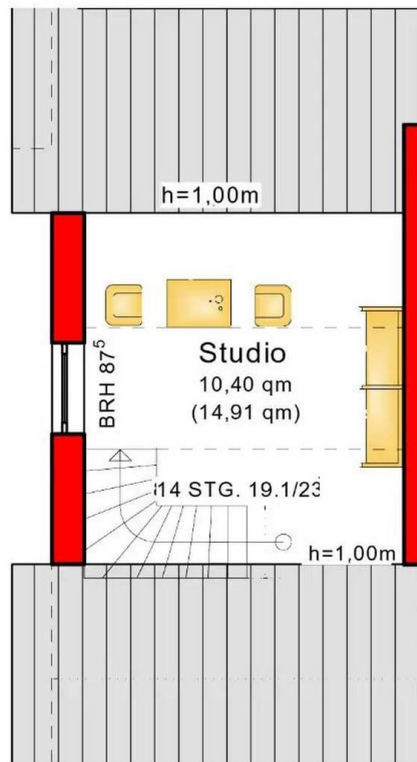
Grundriss Studio
