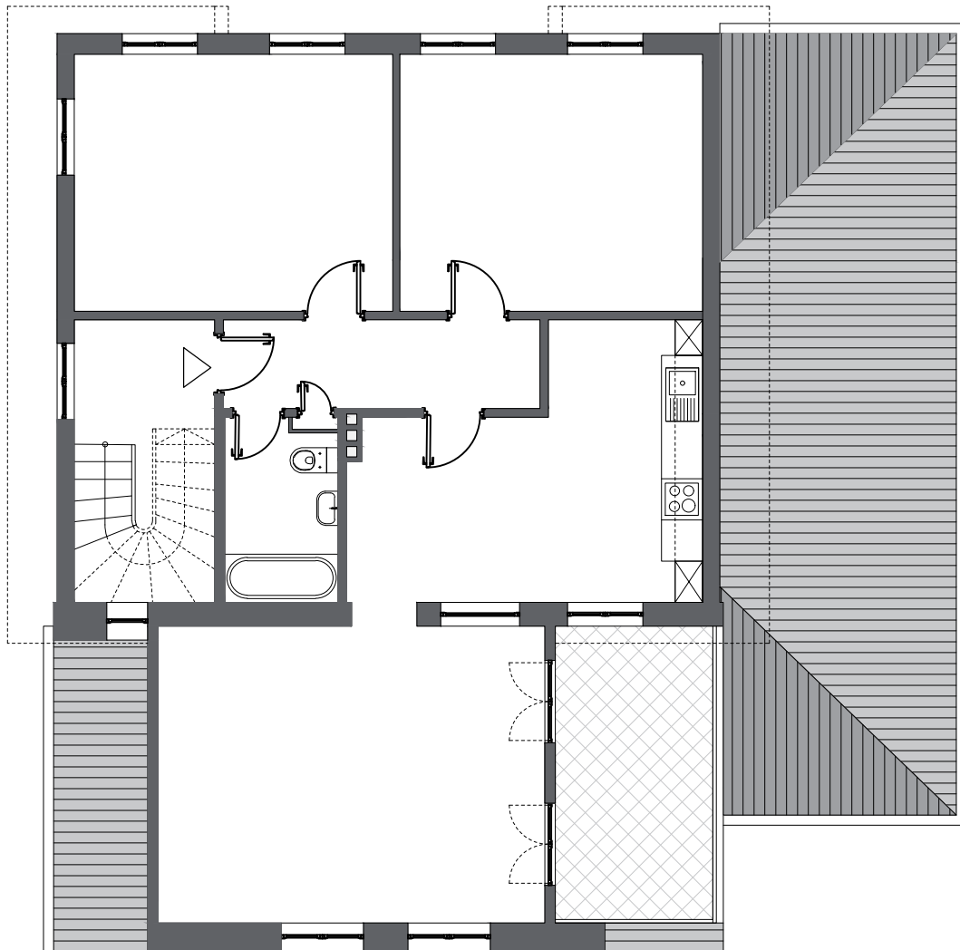
1OG Grundriss
