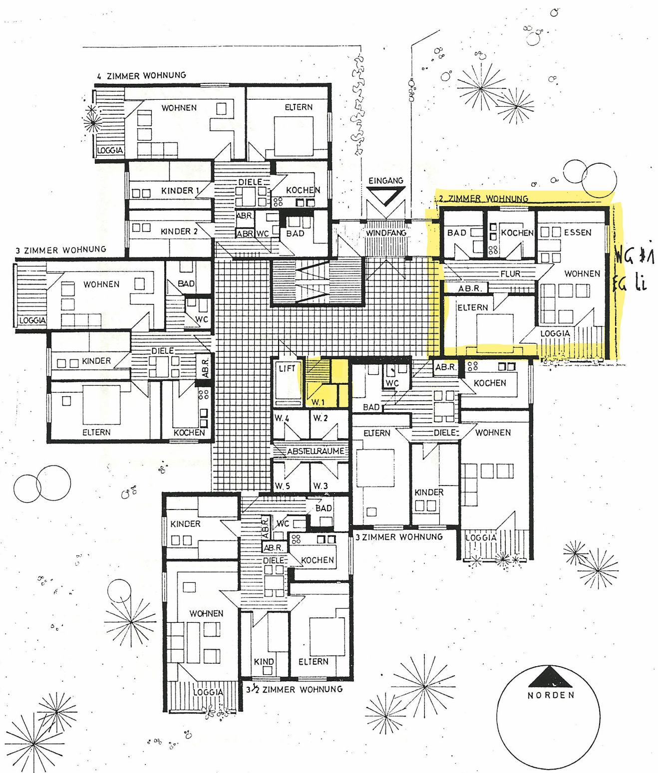
Grundriß Erdgeschoß M = 1 : 200
