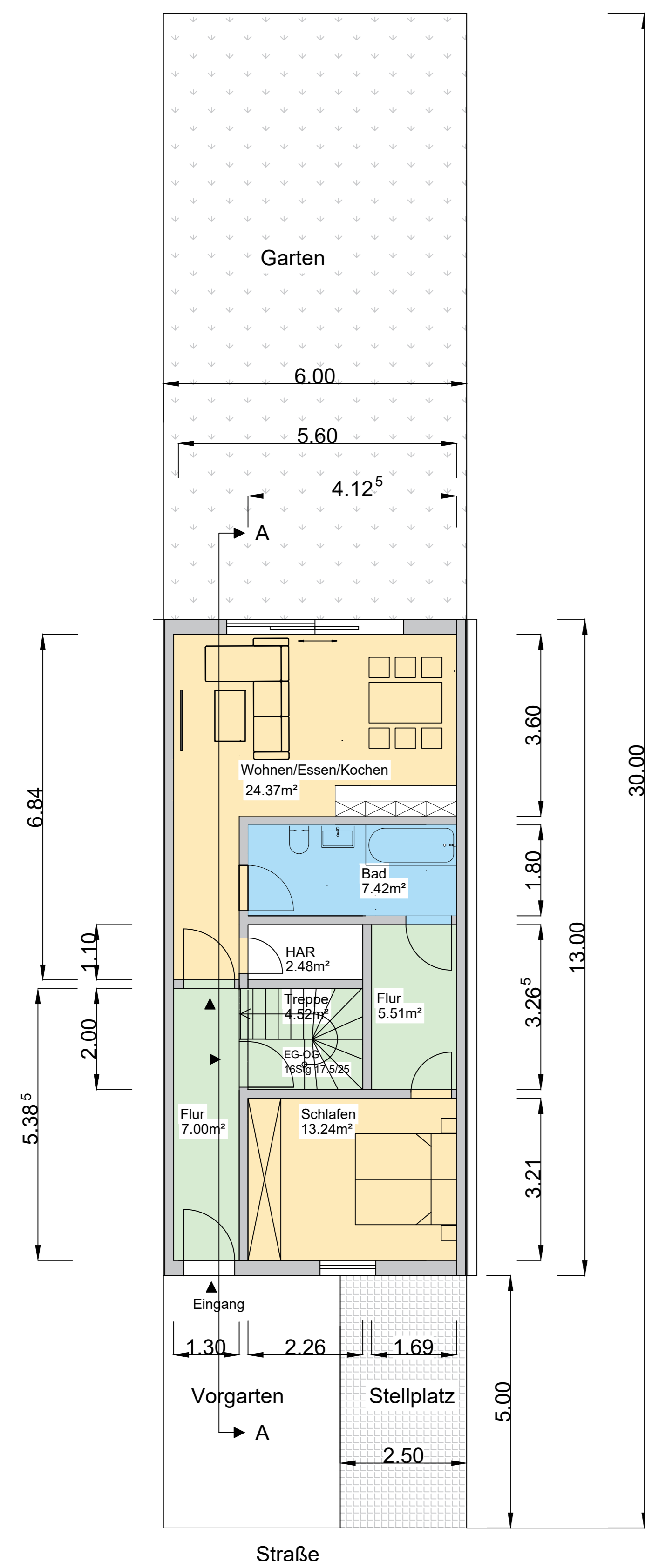
Erdgeschoss 65.73m 2
