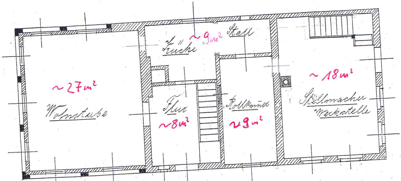
Erdgeschoss.
